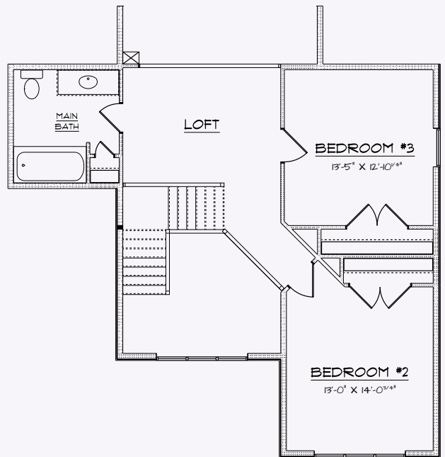
SECOND FLOOR 739 SQFT
