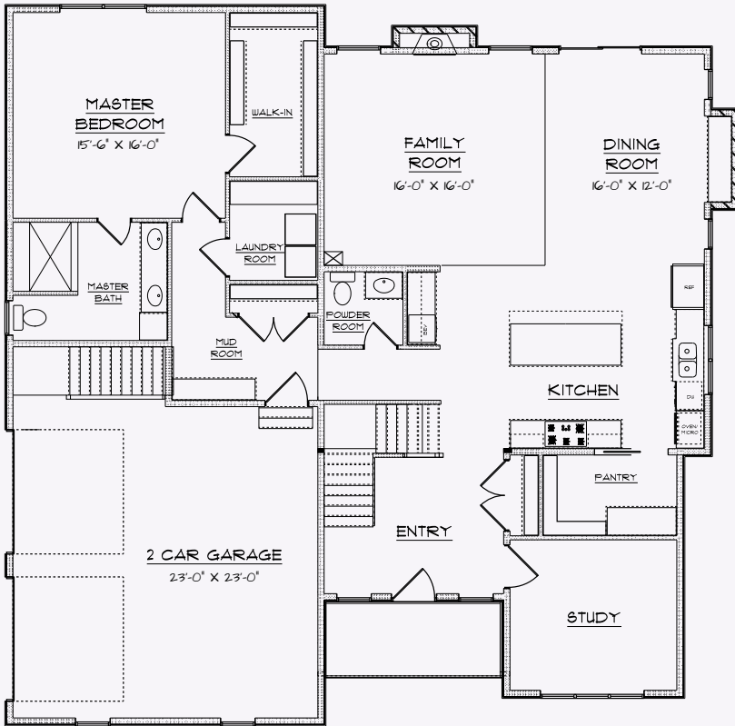
FIRST FLOOR 1835 SQFT
